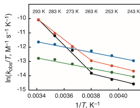
Figure 2. Eyring plots of \ln(k_{\text{obs}}/T) against 1/T obtained in the reactions of 1 with mesitylene (blue circles) and [D 12 ]mesitylene (green circles) and 2 with mesitylene (red circles) and [D 12 ]mesitylene (black circles) at various temperatures (243–293 K).
